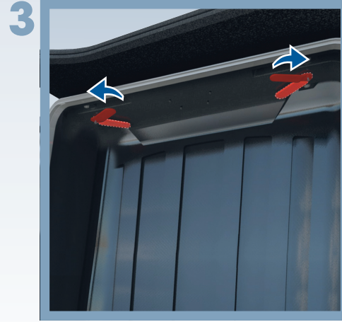
3 Lock the top shelf by turning the two red handles inside the case a quarter of a turn.
